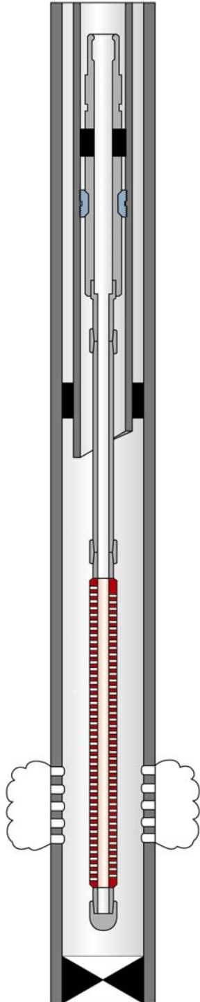
Retrievable Packer
