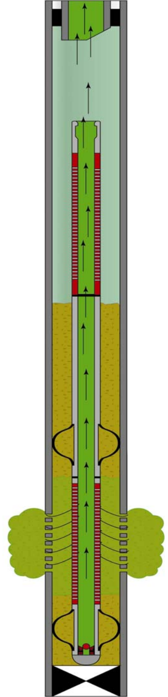
Producing w/Plug Removed
