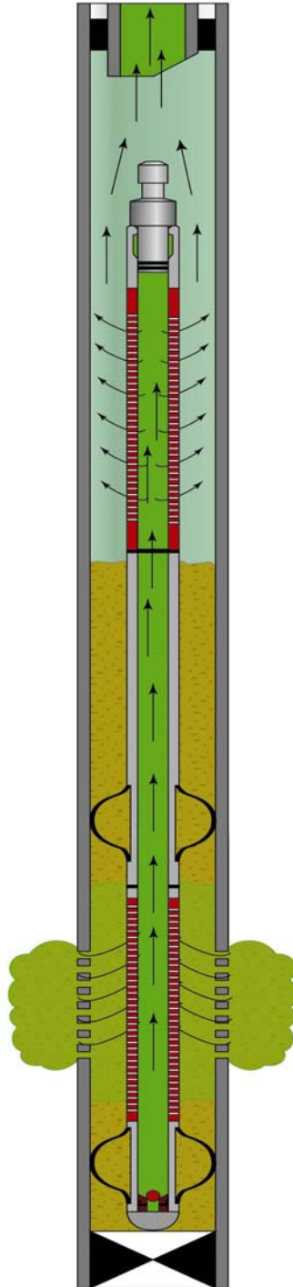
Production w/Plug in Place
