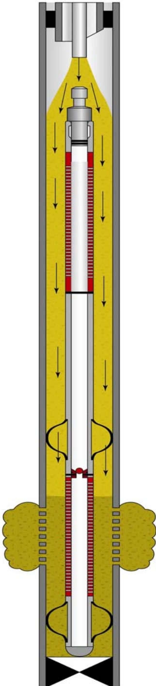
Gravel packing
